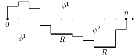
Fig.3. A minimal trajectory containing R -legs.
