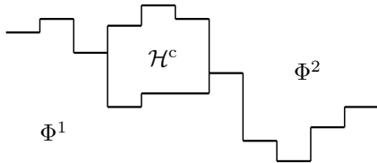
Fig.4. A piece of a trajectory corresponding to \tilde{H}^{(L)} + \delta\tilde{V} .
