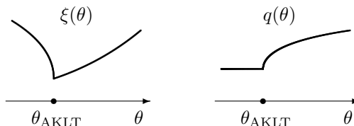
Fig.1. Correlation length \xi(\theta) and incommensurate wave number q(\theta) in a vicinity of the AKLT point.
